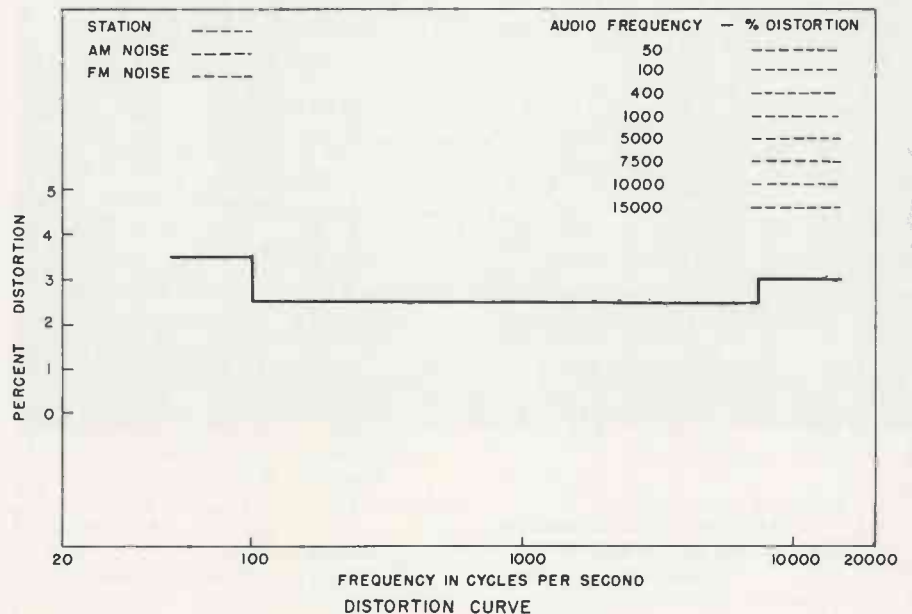
Figure 2C. Typical distortion curve.
