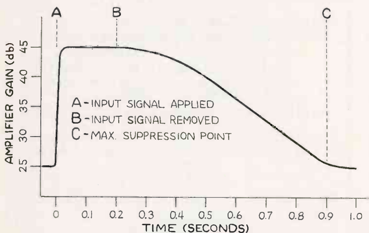
Figure 1. Gate Amplifier Gain Vs. Input Signal.
