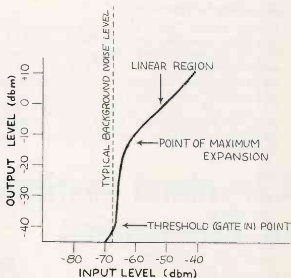
Figure 2. Amplitude Response.
