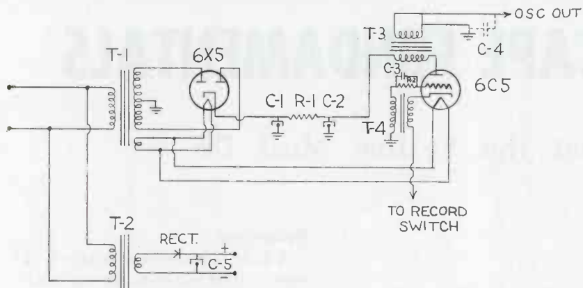
Figure 1 Power supply and oscillator.
