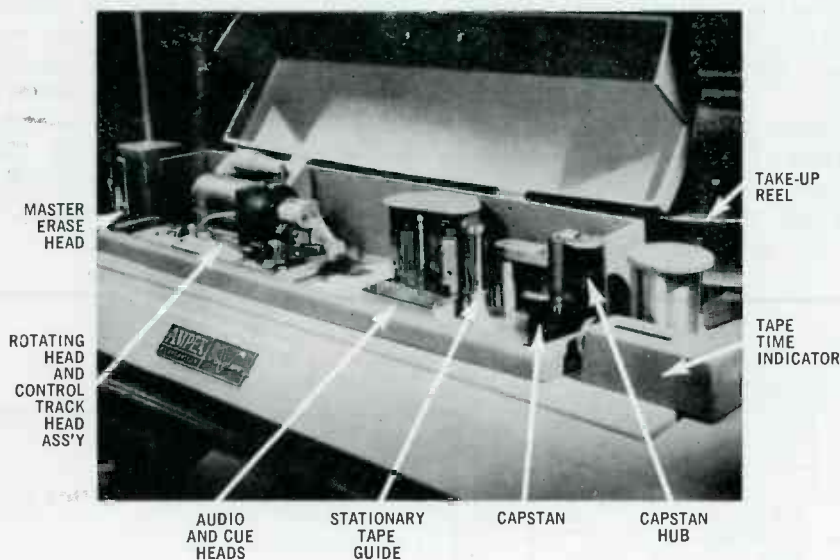
Figure 16* Ampex 1000-B Tape Transport
