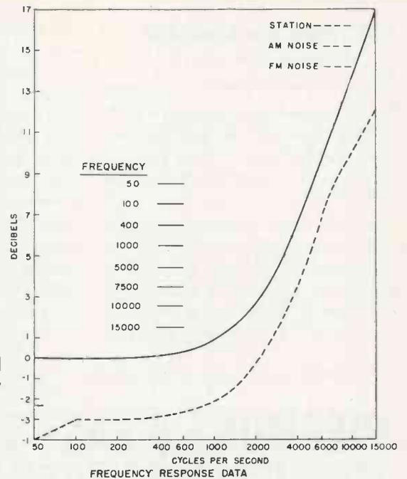
Figure 2B. One method of plotting frequency response data.
