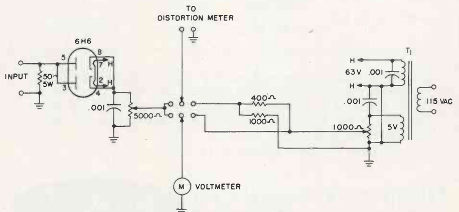
Figure 3. AM noise detector circuit.
