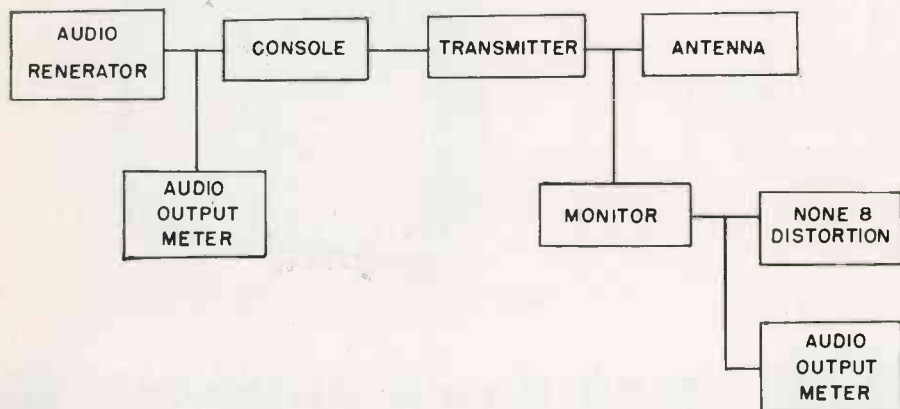
Figure 1. Block diagram of typical proof-of-performance equipment line-up.
