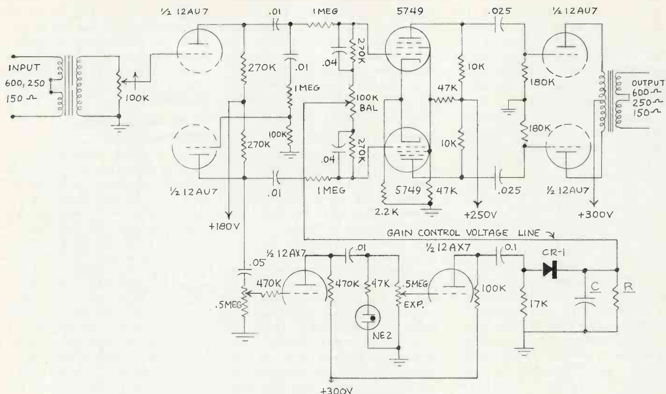
Figure 3. Simplified Schematic.
